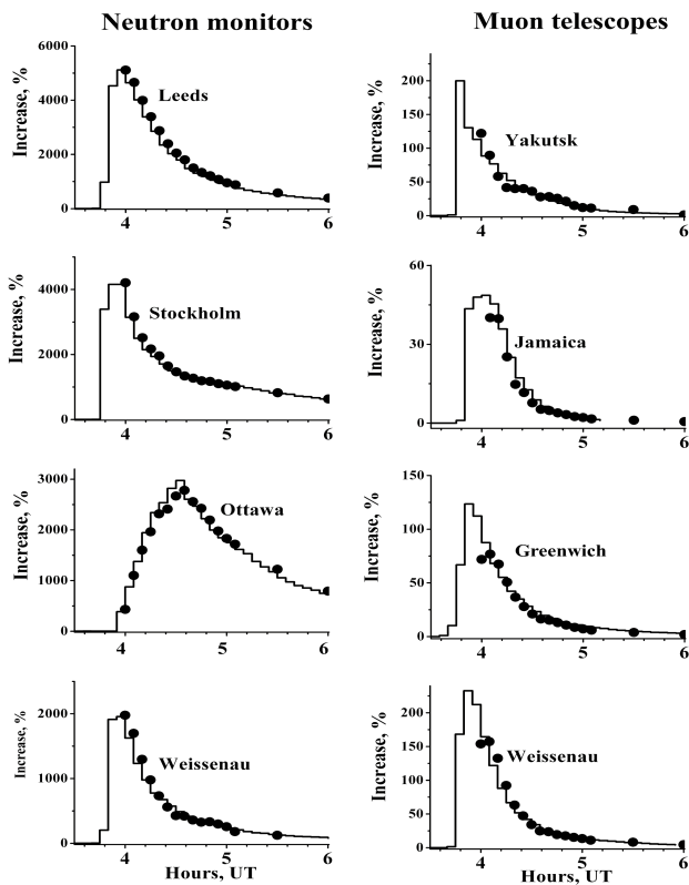
Fig.3. Increase profiles at number neutron monitors (left) and muon telescopes (right) during the GLE 23.02.1956. Points are modeled responses at consecutive 5-minute intervals.
