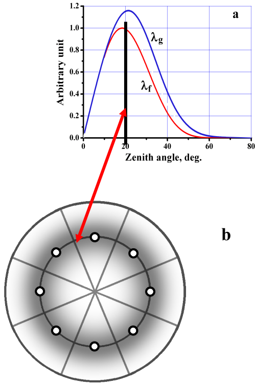
Fig.1. a. Directivity diagram on a zenith angle for GCR ( \lambda_g ) and SCR ( \lambda_f ); b. Launching directions of the 8 inclined trajectories.
