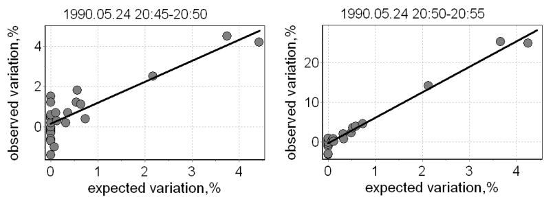
Fig. 2: Comparison of the calculated SN -indices with experimentally observed variations in the GLE event 1990.05.24.
