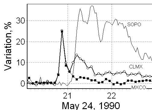
Fig. 1: The count rate variations at the neutron monitors Mexico (MXCO), Climax (CLMX), and South Pole (SOPO) during the GLE on May 24, 1990.
