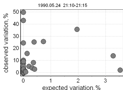
Fig. 4: An absence of correlation between the expected SN -indices and the real enhancement amplitude after the end of neutron signal on 1990.05.24.
