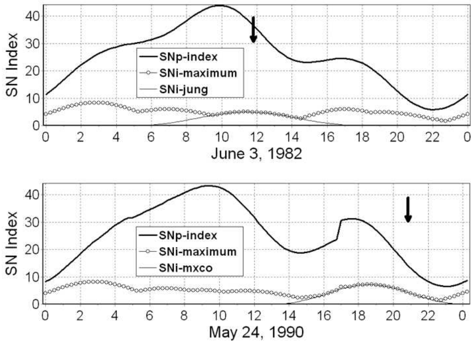
Fig. 5: Behavior of the SN-indices in the two GLE events. The thick curves SN_p correspond to planetary index; arrows mark the maximum of neutron intensity increase at the stations Mexico (above) and Jungfraujoch (below).
