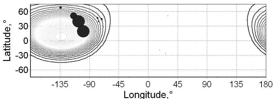
Fig. 3: Distribution of the expected SN -indices calculated for the moment 20:52:30UT 1990.05.24 (isolines), and the observed enhancement values of counting rate in this moment at the neutron monitor stations (black circles; their radius is proportional to the enhancement value).
